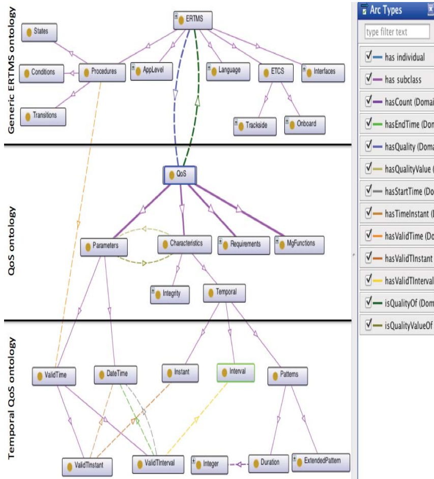
Fig. 4 3-Layer Temporal QoS Ontology for ERTMS/ETCS
