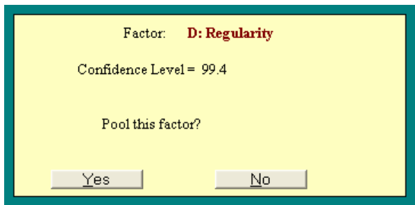
Fig. 5 Test of significance
