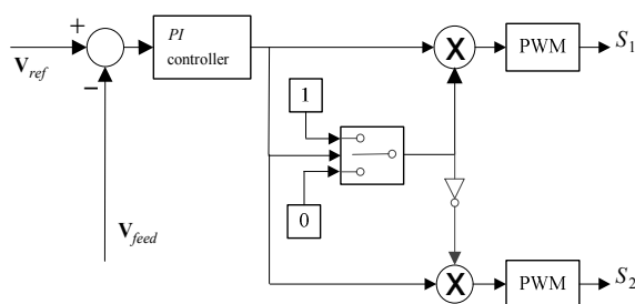
Fig. 5 Control scheme for the proposed inverter
