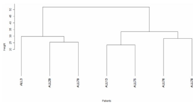
Fig. 6 Hierarchical Clustering of original Affymetrix data (with Euclidean distance and Ward Agglomeration method)
