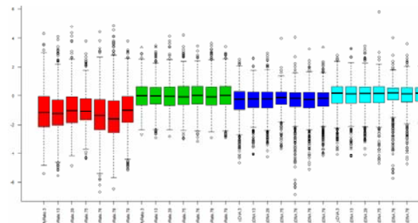
Fig. 5 Boxplots of AffyRatio, cDNA and their respective standard normal distribution
