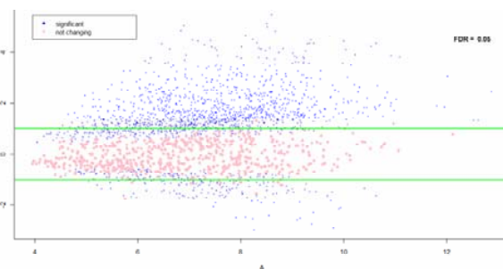
Fig. 3 MA plot comparing healthy and leukaemic samples. Significant genes are the sharp dots, and the horizontal lines are the 2-fold limits.
