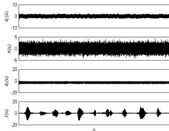
Fig. 4 Decrypted signals
