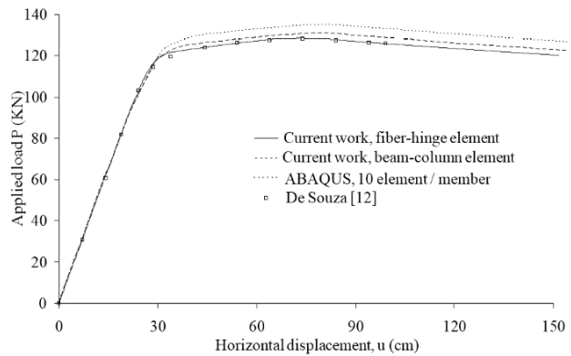
Fig. 9 Load-deflection curves of two-story space steel frame
