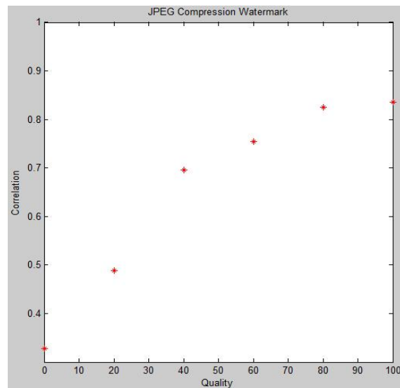
Fig. 15 Correlation due to JPEG compression attacks based on DWT-CT
