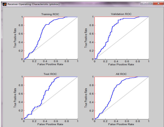
Fig. 13 Receiver operator characteristics curve of the game
