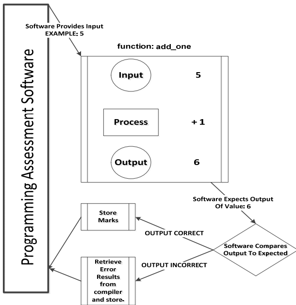
Fig. 2 Assessment logic of PAS
