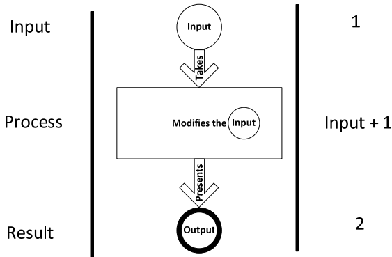
Fig. 1 Input-Process-Output
