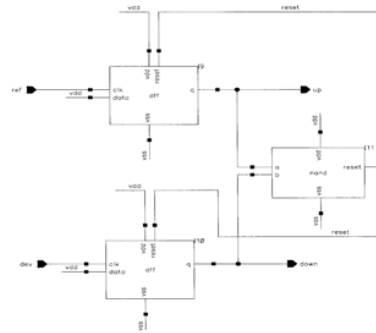
Fig. 9: Phase Detector
