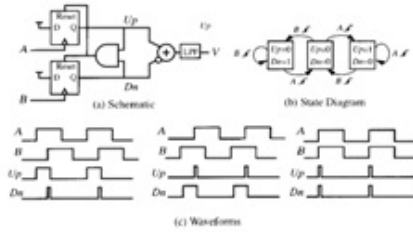
Fig. 3: Phase Detector Waveforms
