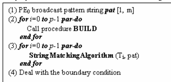
Fig. 1 The distributed string matching algorithm architecture
