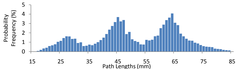
Fig. 4 Path Length Distribution for Different Crowns
