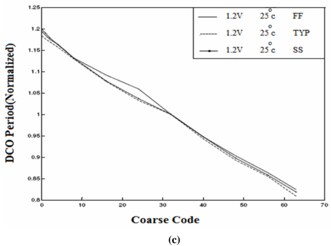
Fig. 8 Delay characteristics of the coarse loop according to Process, Voltage and Temperature variations. (a) Temperature Variation, (b) Voltage Variation, (c) Process Variation
