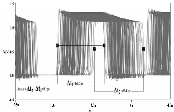
Fig. 11 Time-period jitter of the proposed DCO (Monte Carlo analysis)
