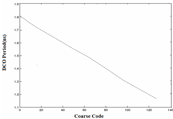
Fig. 10 14-bit DCO structure operating range
