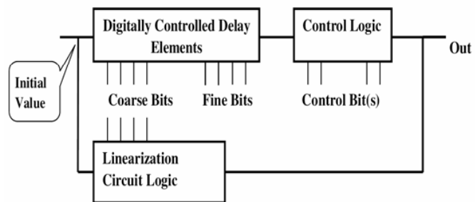
Fig. 1 Block diagram of the ring oscillator DCO
