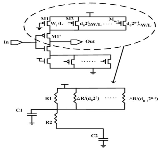
Fig. 3 Equivalent circuit for the calculation of delay tuning range
