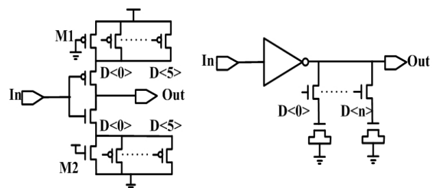
Fig. 2 Standard Cell of Digitally controlled oscillator. (a) Driving strength controlled. (b) Shunt capacitance controlled.
