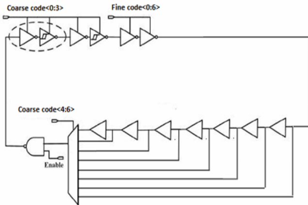
Fig. 9 14-bit proposed DCO structure
