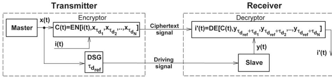
(a) Structure utilizing anticipating synchronization
