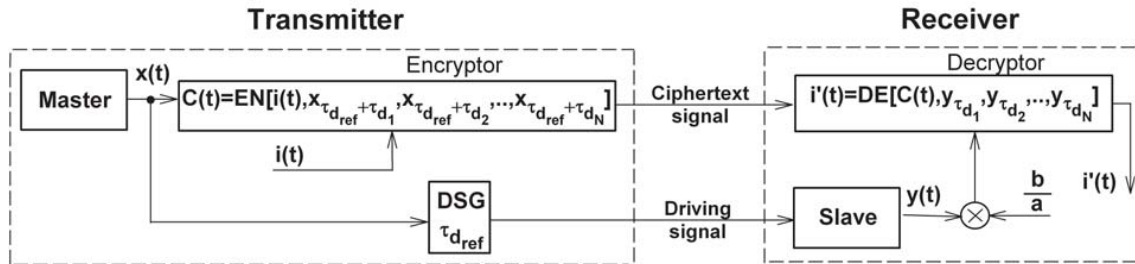
(b) Structure utilizing projective-lag synchronization
