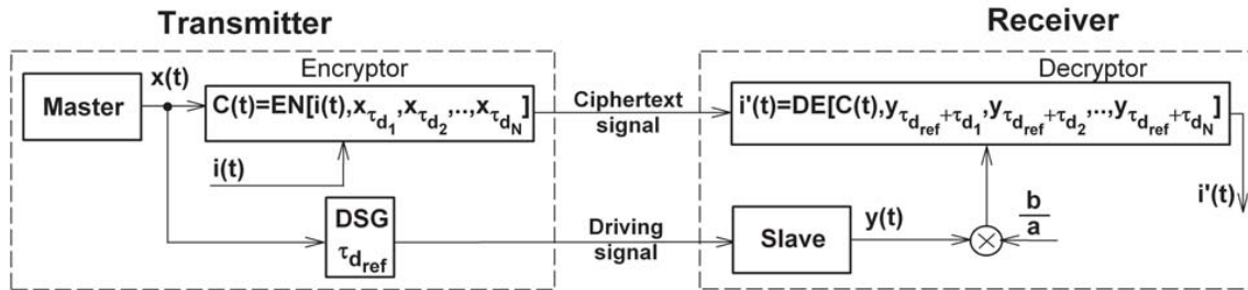
(c) Structure utilizing projective-anticipating synchronization
