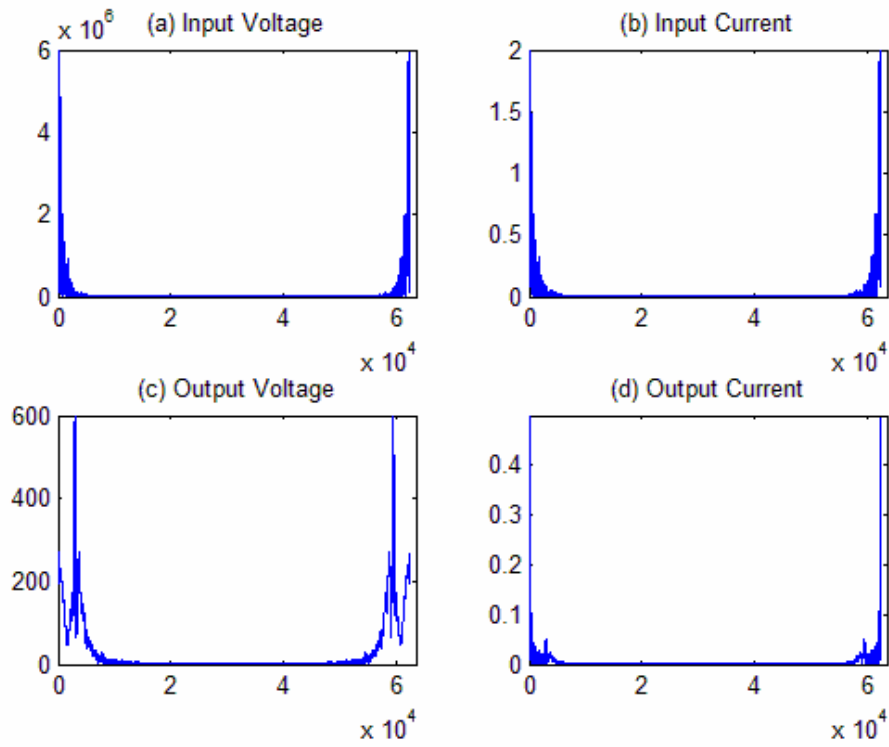
Fig. 4 The first turn of the primary winding is short circuited to the first turn of the secondary winding in with-load mode.
