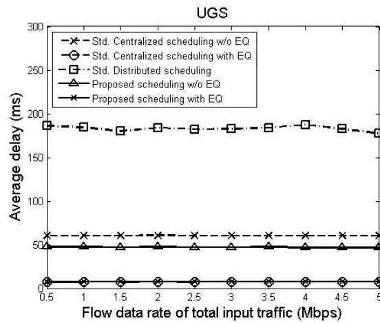
Fig. 7 Average delay of UGS flows
