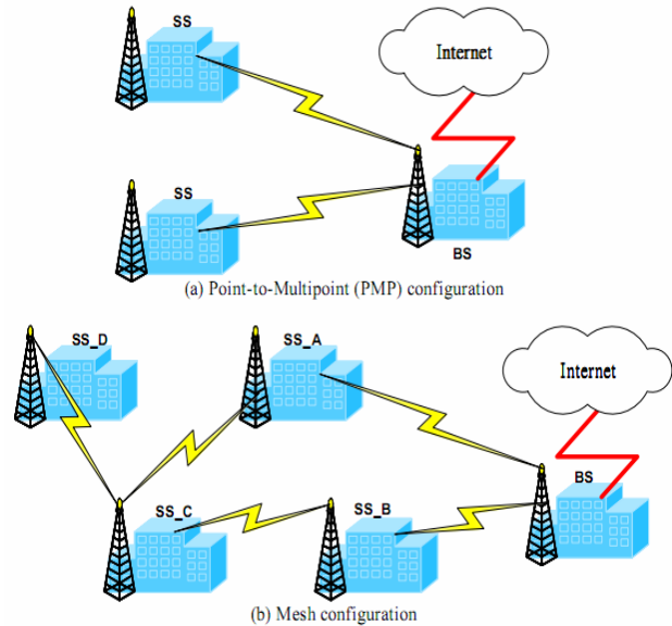
Fig. 1 Two configurations in IEEE 802.16
