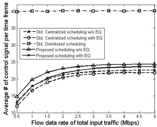
Fig. 13 Average signaling cost
