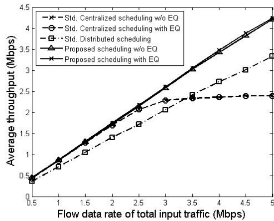
Fig. 12 Average throughput of all flows
