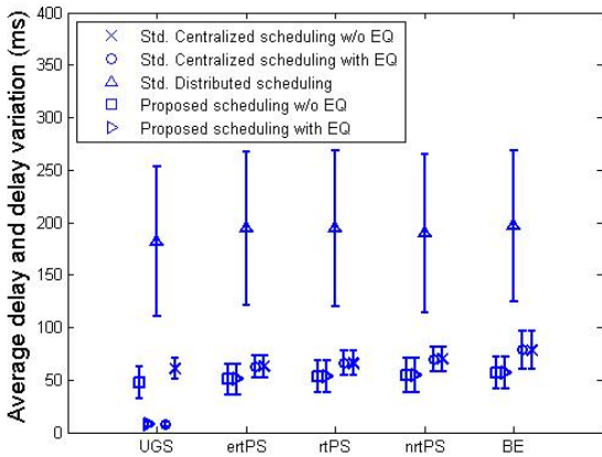
Fig. 5 Delay and delay variation with total flow data rate 2.5 Mbps
