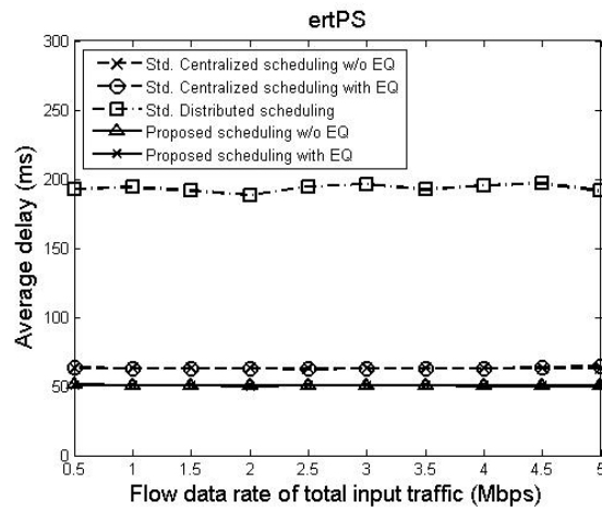
Fig. 8 Average delay of ertPS flows
