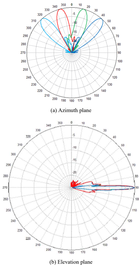
Fig. 5 Radiation patterns of a quad beam antenna covering 120° at 1.8 GHz
