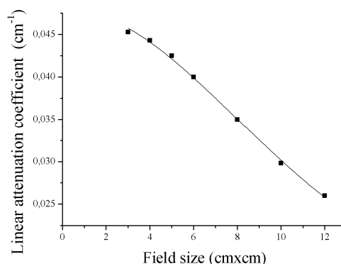
Fig. 2 Linear attenuation coefficient versus field size
