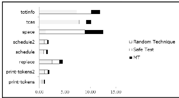
Fig. 6 The comparison of finding faults
