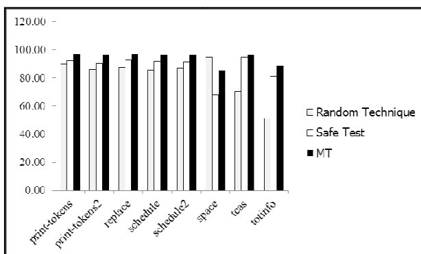
Fig. 5 The reduction of the comparison techniques
