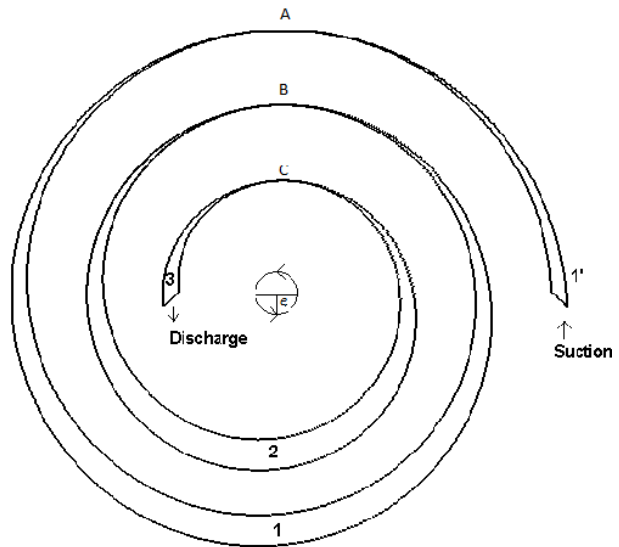
Fig. 2 Relative position of two spirals for an intermediate crank angle showing various gas pockets
