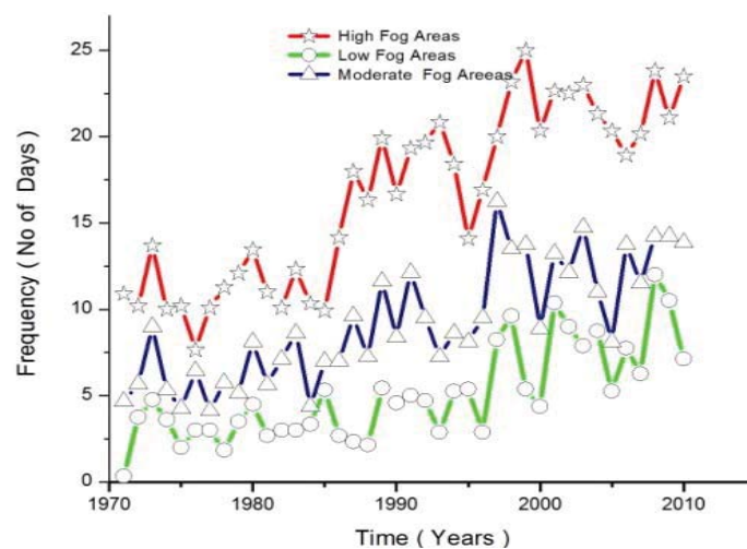
Fig. 6 Time series analysis -fog prone zone wise
