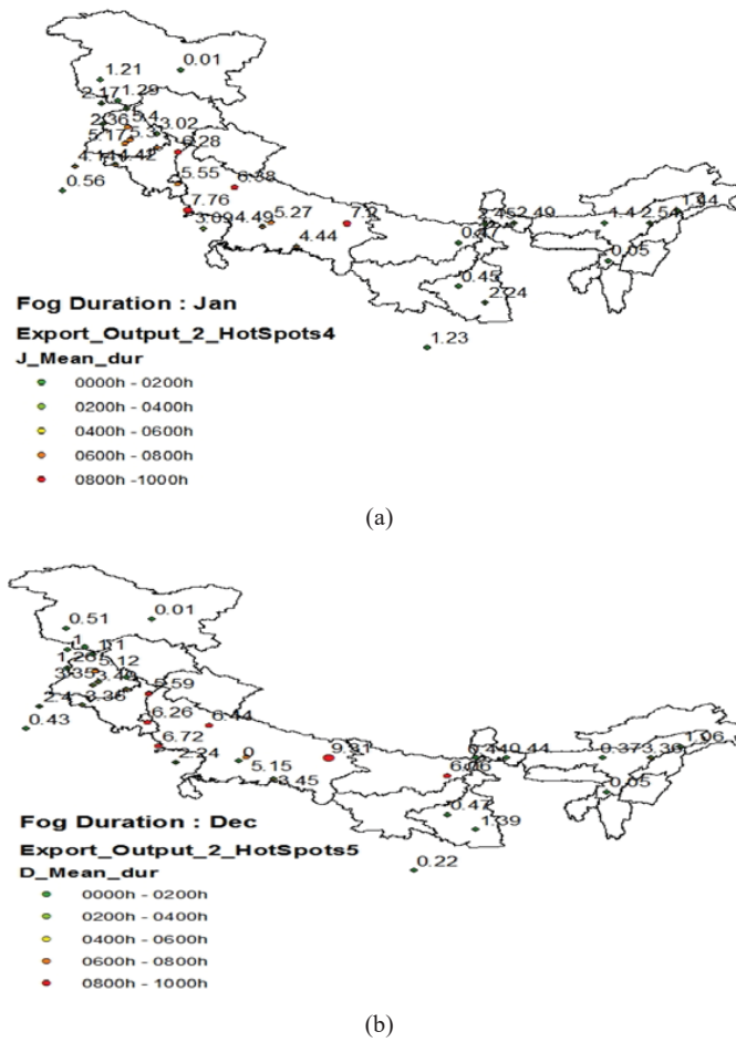
Fig. 13 (a) Average Daily Persistence (January), (b) Average Daily Persistence (December)
