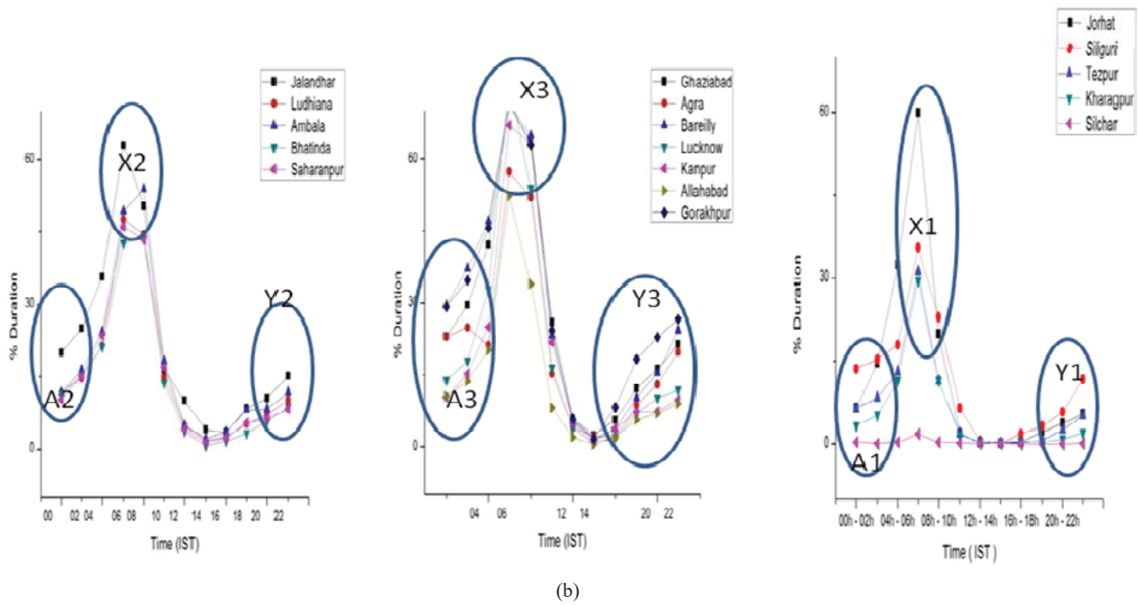
Fig. 12 (a) Diurnal Variability(Jan), (b) Diurnal Variability (Dec)
