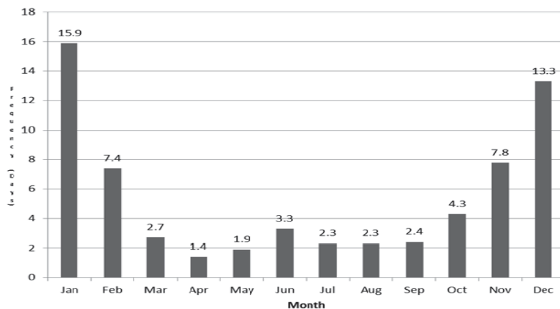
Fig. 2 Average Monthly Visibility (less than 1 km in days)
