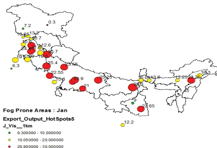
Fig. 3 Fog Classification (Hot spot Analysis)
