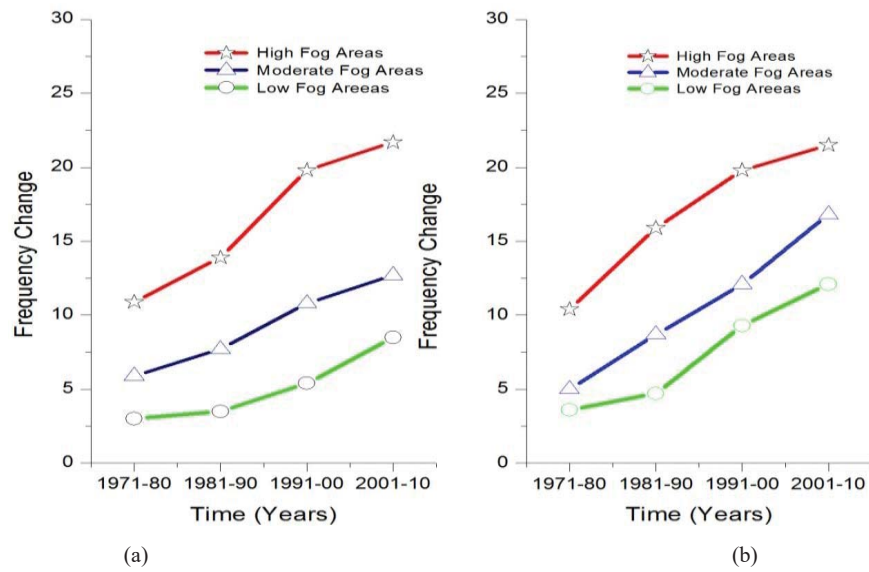
Fig. 11 (a) Decadal change in fog frequency (January), (b) Decadal change in fog frequency(December)
