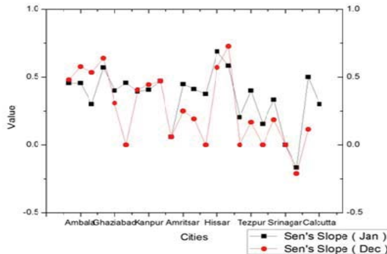
Fig. 9 Theil and Sen's Slope
