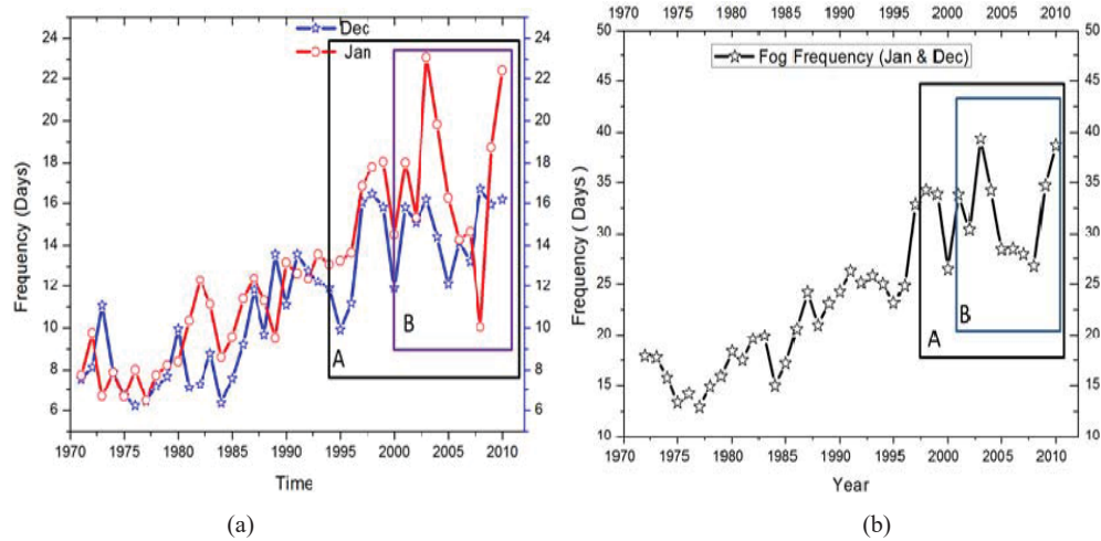
Fig. 5 (a) Time series Analysis (Dec &amp; Jan), (b) Time series Analysis (winter season)
