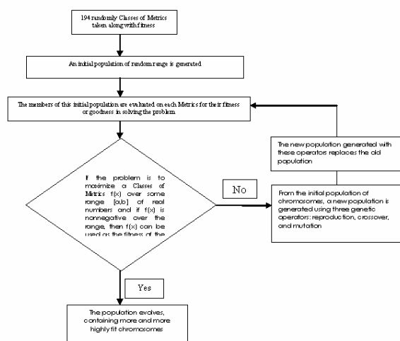
Fig. 1 Flowchart of use of GA
