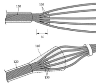
Fig. 2 Improvement of bond characteristics
