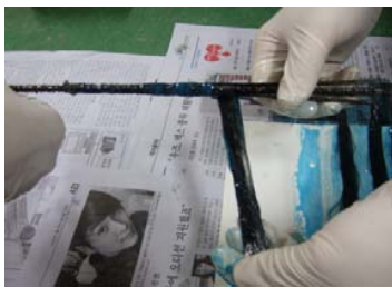
Fig. 4 Fiber reinforcement
