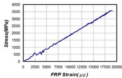
Fig. 6 Load-displacement curve
