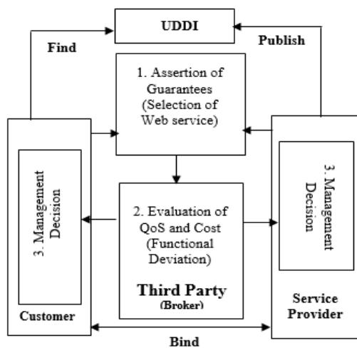
Fig. 1 AWMC Framework
