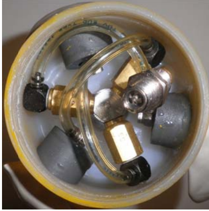
Fig. 5 Flotation system
