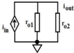
Fig. 5 Common Gate amplifier when R_{load} is cascode load.
