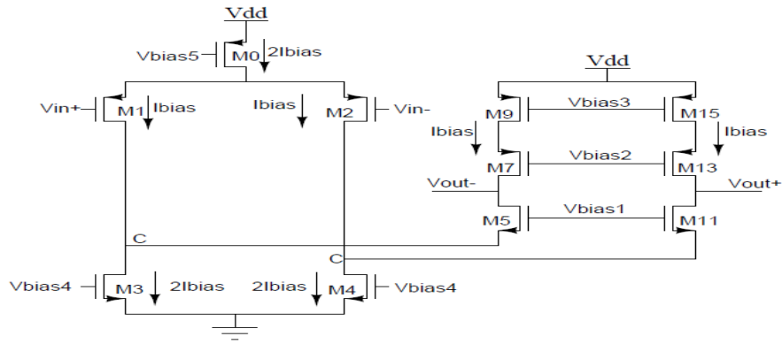
Fig. 1 Folded Cascode OTA
