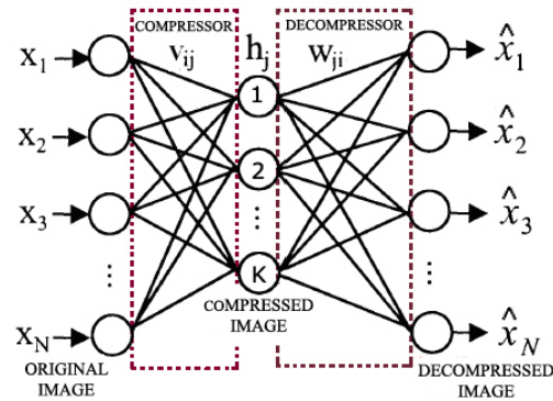
Fig. 1 Basic image compression structure using neural network
