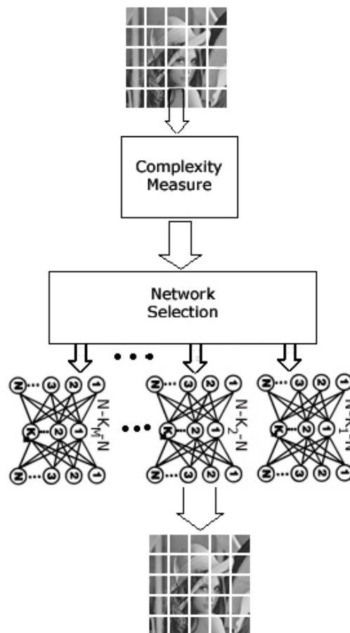
Fig. 2 Neural network-based adaptive structure for image compression
