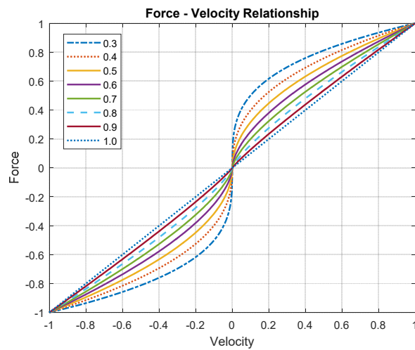
Fig. 2 Force-velocity relationship for various values of \alpha
