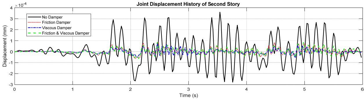
Fig. 13 Joint Displacement History of Second Story
