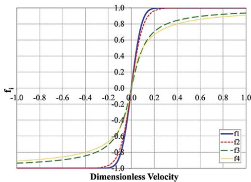
Fig. 5 Force velocity relationships according to Mostaghel and Davis [9]
