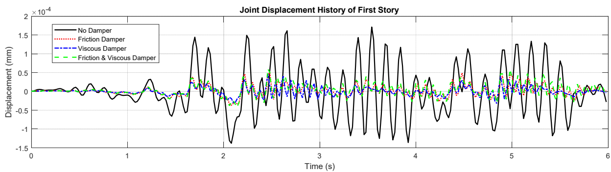
Fig. 12 Joint Displacement History of First Story
