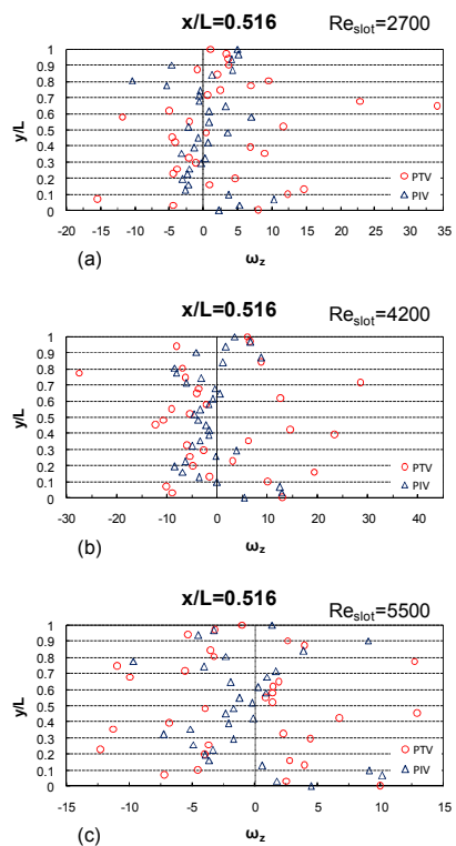
Fig. 9 Z-vorticity profiles at X/L=0.516
