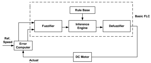
Fig. 3 Fuzzy logic Controller
