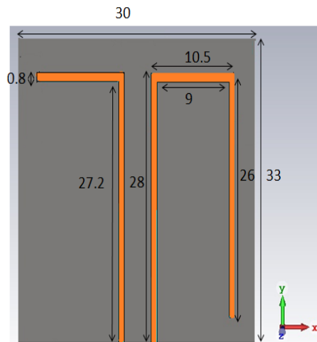
Fig. 1 Geometry and dimensions of the proposed wideband slot antenna (the grey shaded area represents the metallization)
