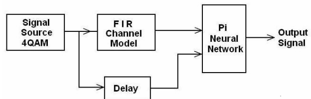
Fig. 1 A digital communication system model
