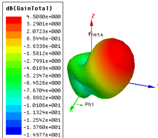
Fig. 12 Gain at 9.17 GHz
