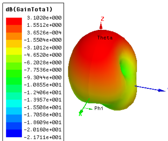
Fig. 13 Gain at 10.45 GHz
