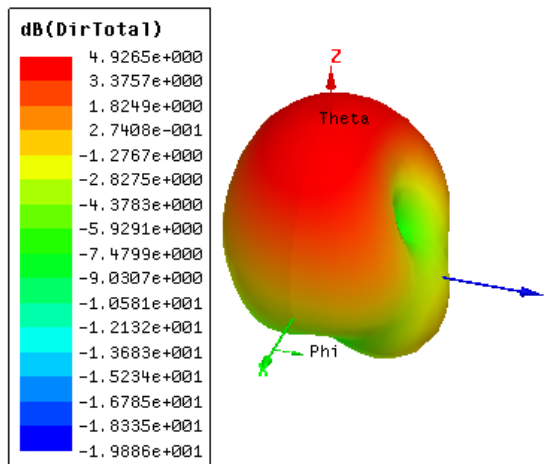
Fig. 17 Directivity at 10.45 GHz
