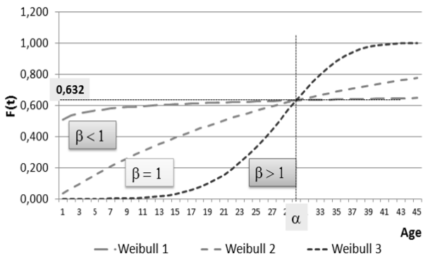
Fig. 2 Weibull reliability functions: Cumulative failure
