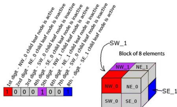
Fig. 4 Unsigned byte flag example
