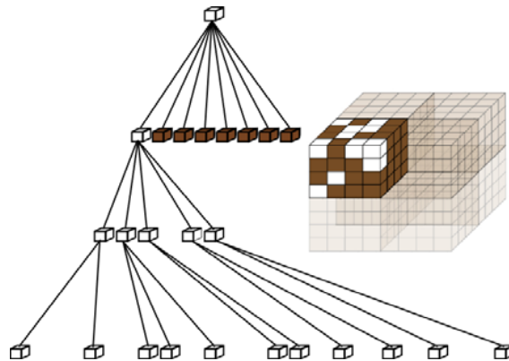
Fig. 2 Octree structure example
