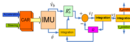
Fig. 3 INS mechanization equations in 2 D
