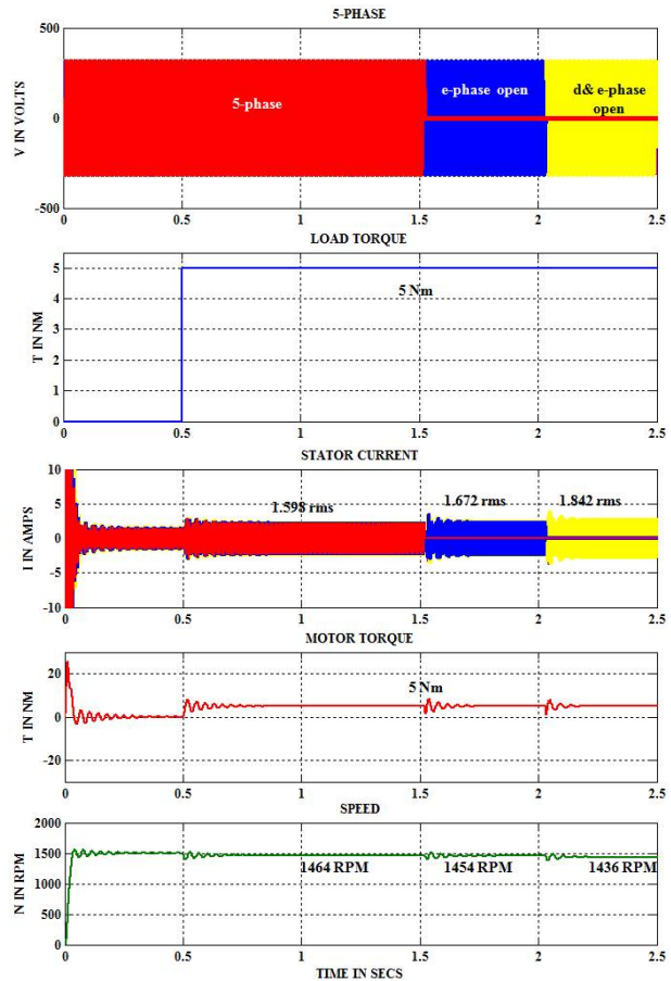
Fig. 9 Five-phase induction motor with one and two of the phases opened
