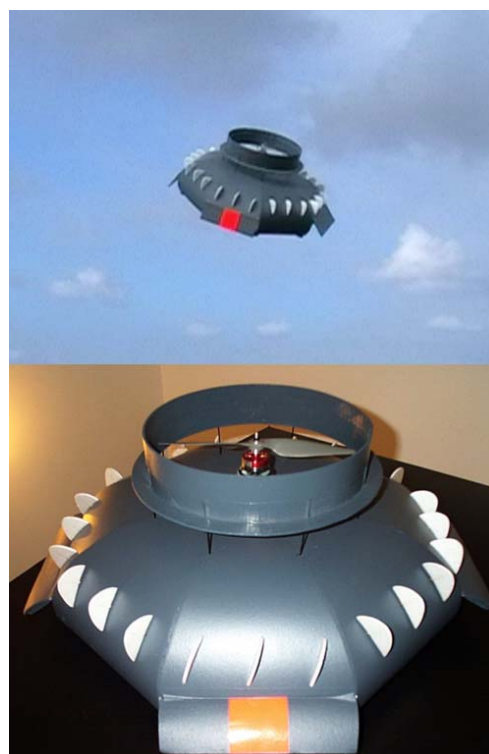
Fig. 1 A typical Coanda Saucer UAV developed and tested by Jean-Louis Naudin. The diameter of the saucer is approximately 60 cm [11]
