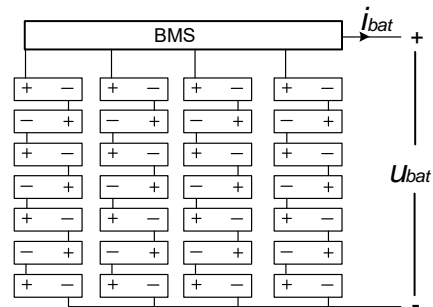
Fig. 1 Schematic battery layout
