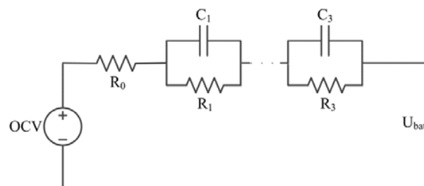
Fig. 4 EEC model
