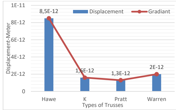
Fig. 8 Curve of the maximum displacement values in trusses under cyclic load
