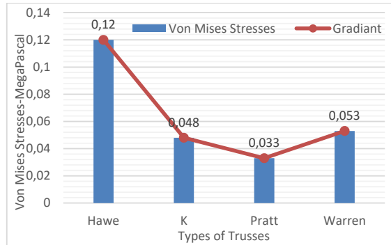
Fig. 6 Curve of the maximum amount of stress of the Mens von in the trusses under a cyclic load
