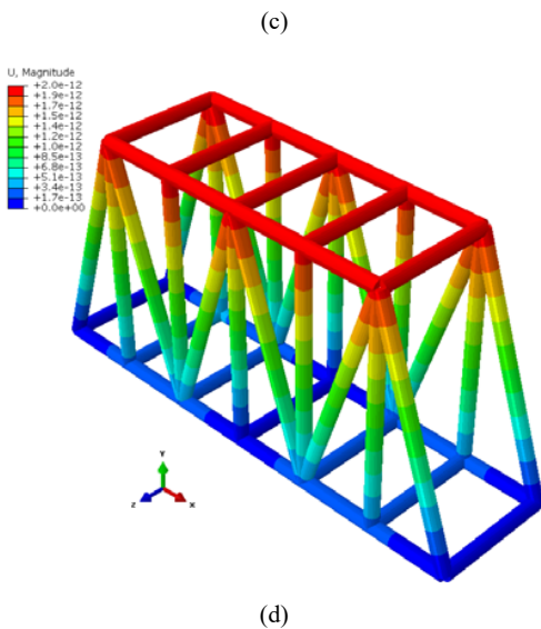
Fig. 7 Displacement in trusses a) Hawe, b) K, c) Pratt and d) Warren under cyclic load
