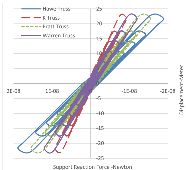
Fig. 15 Hysteresis curve in trusses under cyclic load
