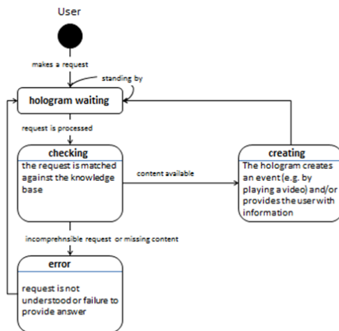
Fig. 6 The OLOS® Event Manager flow diagram
