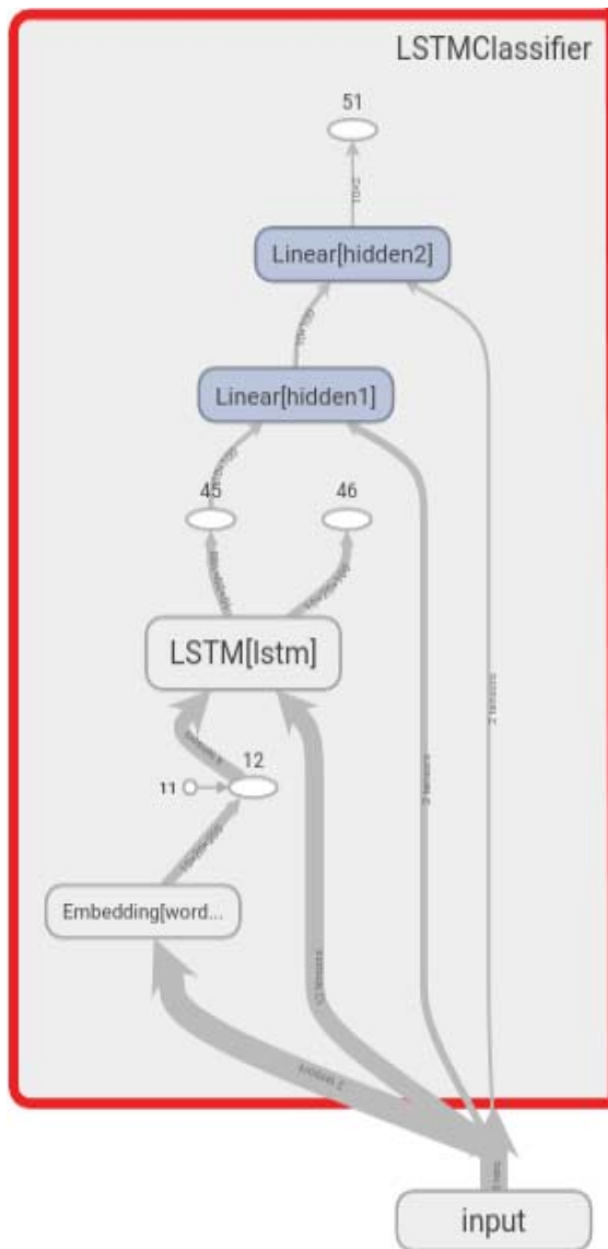
Fig. 2 LSTM architecture
