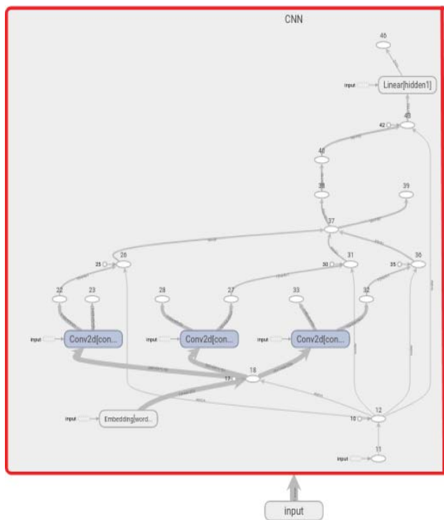
Fig. 1 CNN architecture
