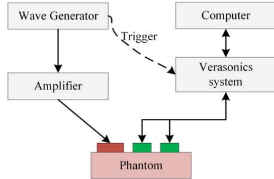
Fig. 2 The circular element and two rectangular elements are used to generate and track shear waves respectively
