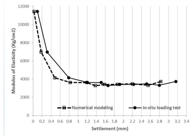
Fig. 8 Modifications of the elasticity modulus against the settlements for numerical modeling and in-situ loading test
