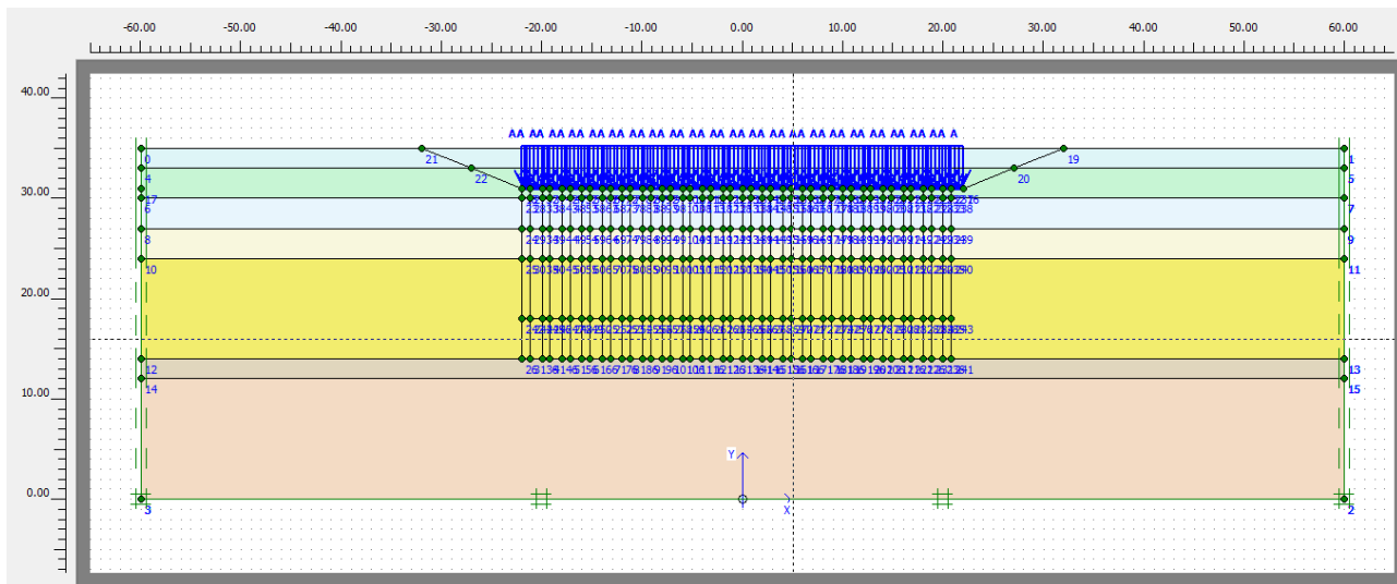
Fig. 6 Numerical modeling in PLAXIS software using in-situ loading test
