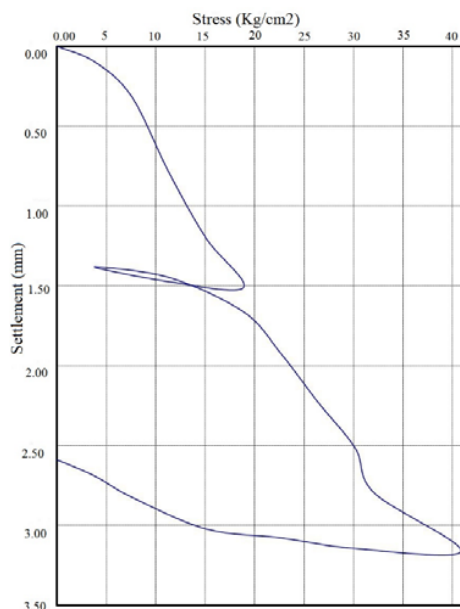
Fig. 4 Typical results of static loading test
