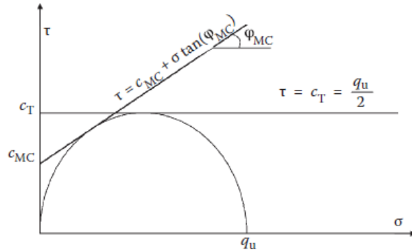
Fig. 1 Two proposed failure models for JG columns
