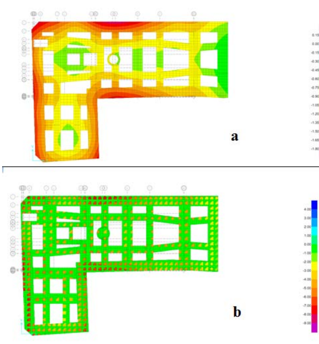
Fig. 5 The status of stresses below the foundation under the service load (a) before the improvement, (b) after the improvement
