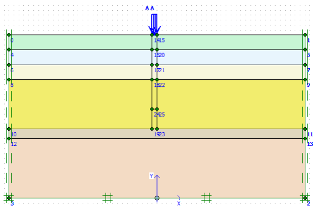
Fig. 7 Numerical modeling in PLAXIS software for a column JG
