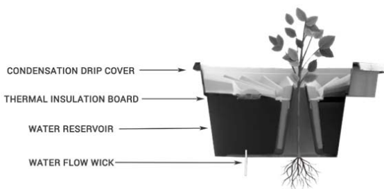
Fig. 1 Ekobox supporting unit
