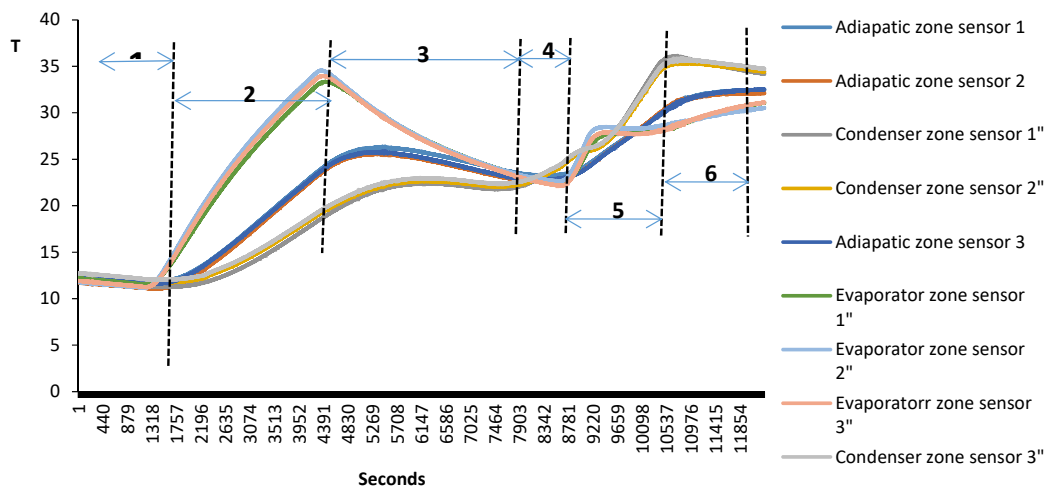
Fig. 31 Testing algorithm
