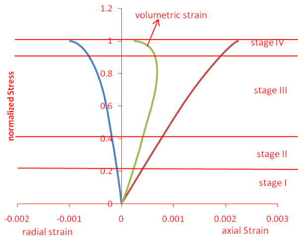
Fig. 8 Normalised stress-strain curves, Troctolite specimen
