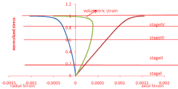
Fig. 4 Normalised stress-strain curves, Marble specimen
