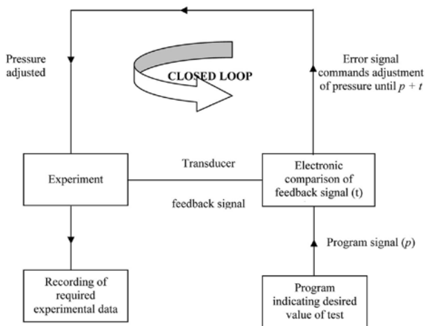
Fig. 1 Principles of closed-loop servo-controlled system [6]
