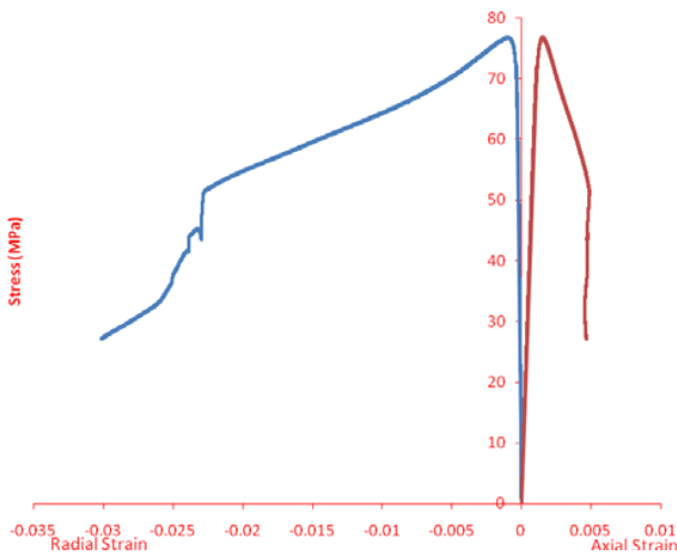
Fig. 5 Post-failure stress-strain curves, Marble specimen
