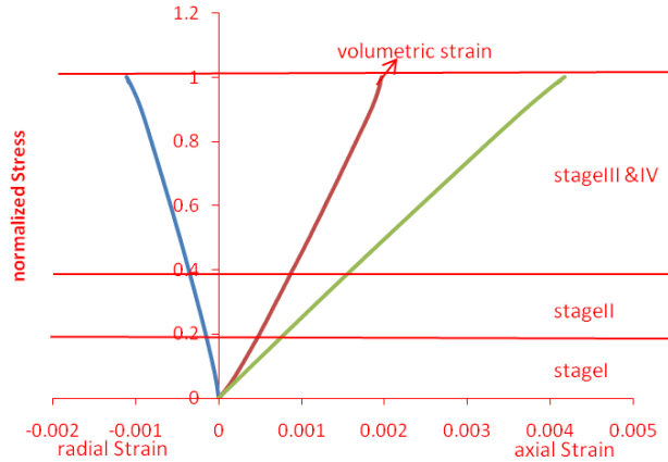
Fig. 12 Normalised stress-strain curves, Gabbro specimen
