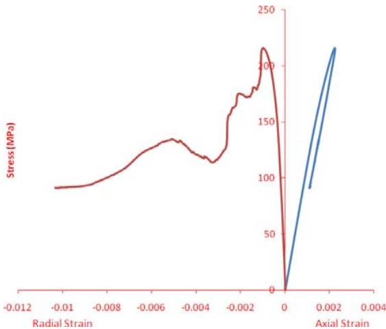
Fig. 9 Post-failure stress-strain curves, Troctolite specimen
