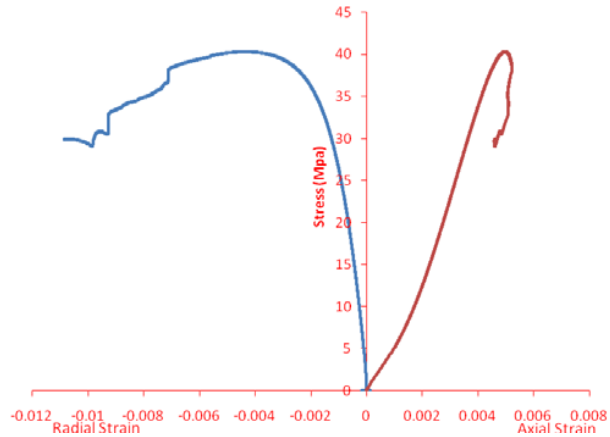
Fig. 7 Post-failure stress-strain curves, Sandstone specimen
