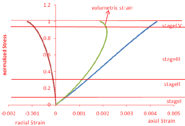
Fig. 10 Normalised stress-strain curves, Quartzite1 specimen
