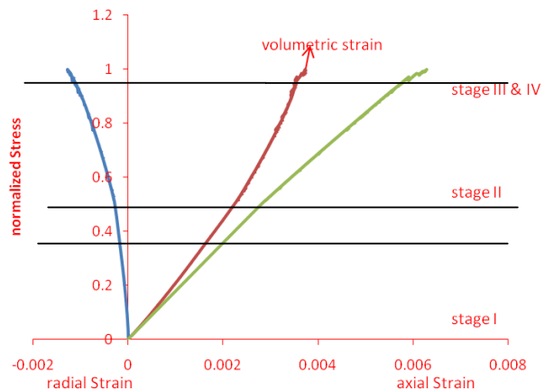
Fig. 13 Normalised stress-strain curves, Quartzite2 specimen
