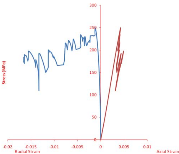
Fig. 11 Post-failure stress-strain curves, Quartzite1 specimen
