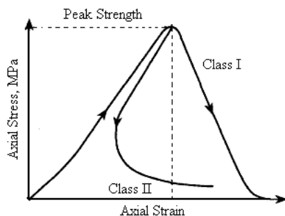
Fig. 2 Classification of rocks based on post-failure characteristic behaviour in compression [9]
