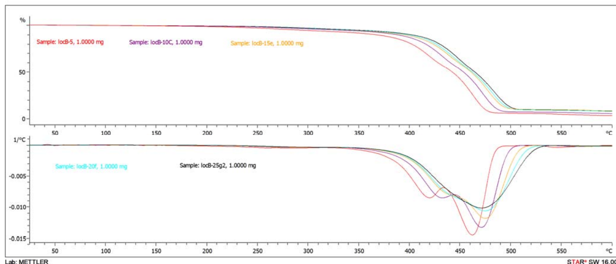
Fig. 3 TGA Result of the PSW Sample
