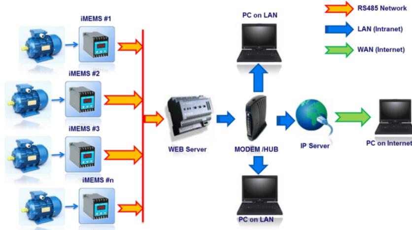
Fig. 4 Block diagram of the developed system
