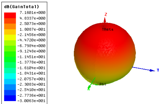
Fig. 4 3D Gain plot for Conventional Antenna
