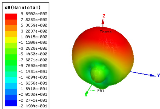
Fig. 8 3D gain plot for 2X1 antenna array
